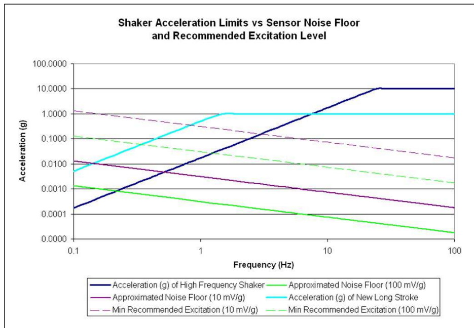
Reference The Modal Shop's Sensor & Cal Tips #43 - Long Stroke Precision Calibration Exciter
